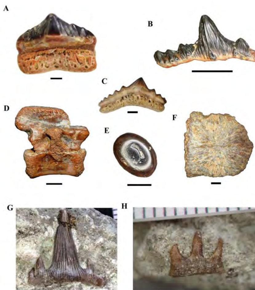
Figure 1. A-F : Shark and aquatic reptile remains from Holwell (Rhaetian, Late Triassic). A) M64, Tooth of Lissodus minimus in lingual view; B) M192, Tooth of Hybodus cloacinus in labial view; C) M183, Lateral tooth of Synechodus rhaeticus in lingual view; D) C28, vertebra of Pachystropheus
